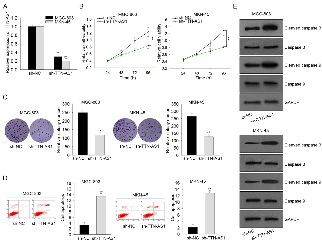
Figure 2. Silencing of TTN-AS1 inhibited cell proliferation and facilitated apoptosis in gastric cancer. A ) qRT-PCR assay was utilized to investigate the expression level of TTN-AS1 in MGC-803 and MKN-45 cells transfected with sh-TTN-AS1 or sh-NC. B–C ) The effect of TTN-AS1 knockdown on MGC-803 and MKN-45 cells proliferation was detected by MTT assay and colony formation assay. D ) Flow cytometry assay revealed the cell apoptosis in MGC-803 and MKN-45 cells transfected with sh-TTN-AS1. E ) Western blot analysis showed the protein levels of total caspase 3, cleaved caspase 3, total caspase 9 and cleaved caspase 9 in MGC-803 and MKN-45 cell lines. * p<0.05 , ** p<0.01 .
